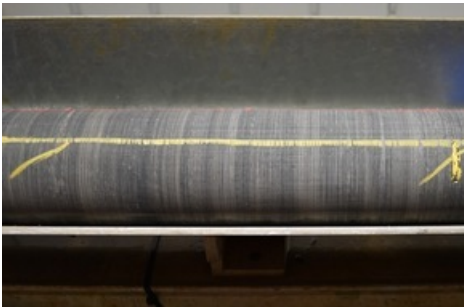
Bohrkern Opalinuston
